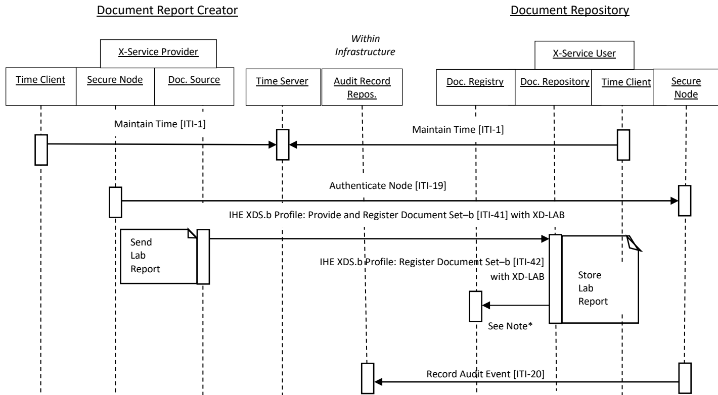
FIGURE 4.2.1-1 CODED LABORATORY RESULTS SEQUENCE DIAGRAM (1)
